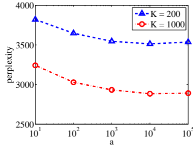
Figure 2: Sensitivity analysis with respect to difference prior strength a .
